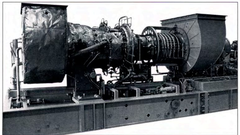
A Wahlco thermocouple harness monitors the exhaust gas temperature of this gas turbine package.
