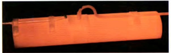
Thermocouple testing at 2100°F. The thermocouples are mounted on a boiler tube shield; the thermocouple on the left is measuring temperature near the tube shield; the (tubeskin) thermocouple on the right is directly measuring tube shield temperature.
