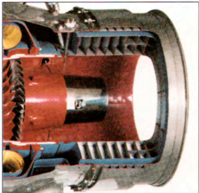
Thermocouple probes are used in the exhaust duct of this aviation auxiliary power unit (APU).
