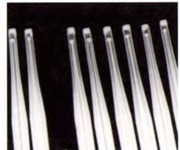
Radiograph inspection of ungrounded tapered thermocouples. Diameters are 0.125," swaged to 0.063," with Inconel® 600 sheaths for gas turbine exhaust duct measurement.
